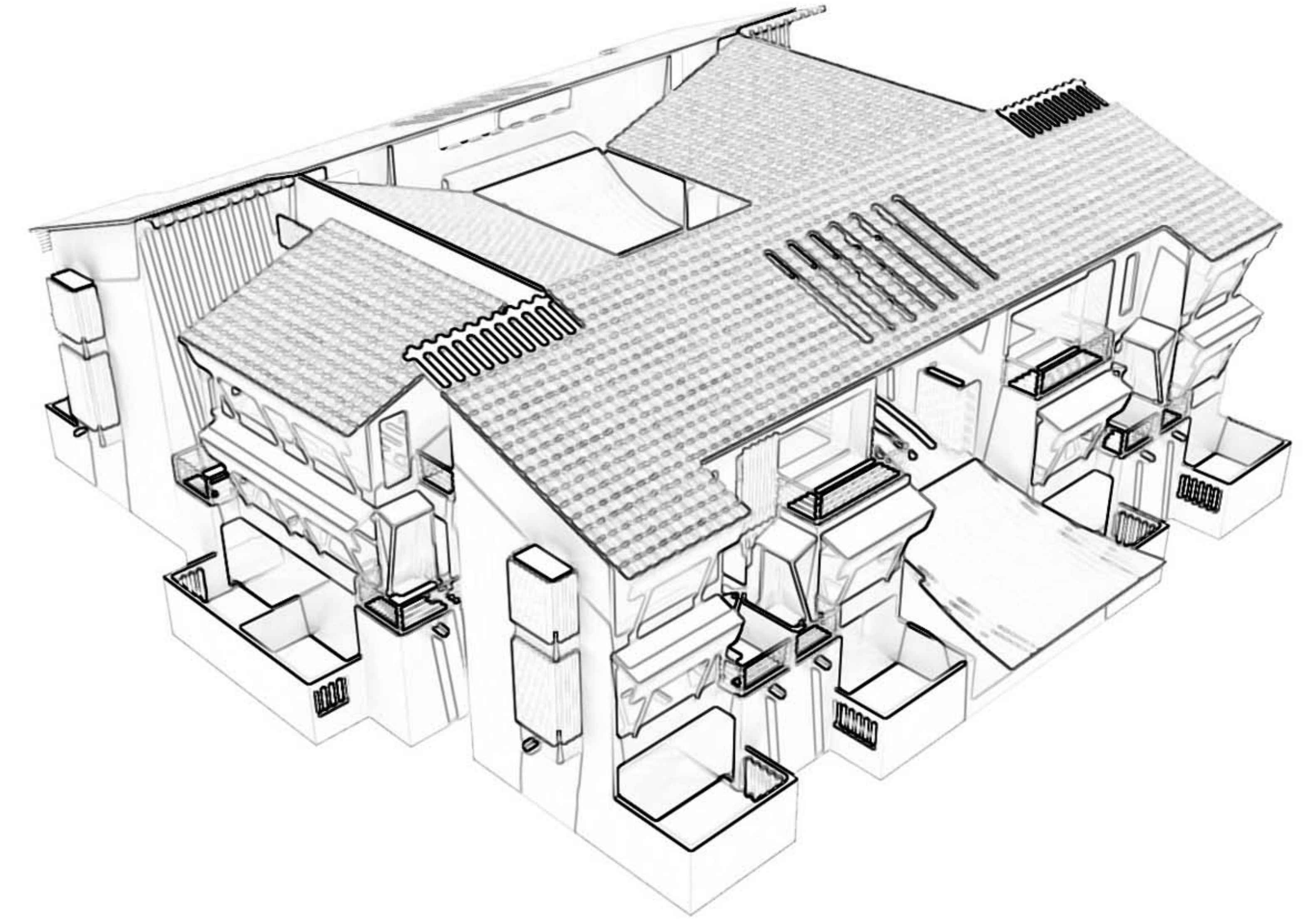
DESIGN DEVELOPMENT : GUEST HOUSE
